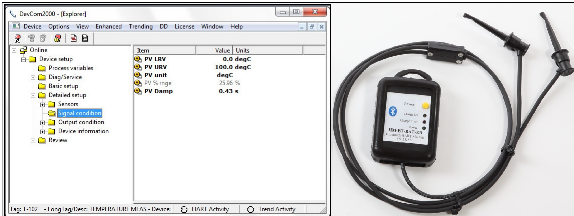
DevCom2000 HART Software + HM-BT-BAT-ER Bluetooth HART Modem
