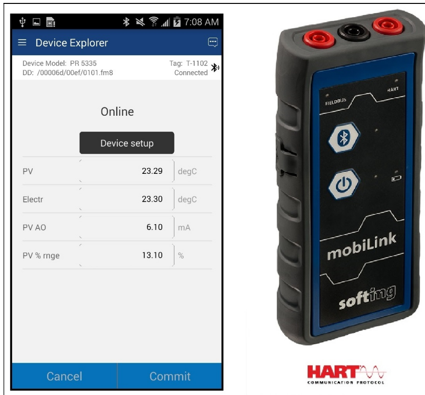
DevComDroid HART App + MOBI-HART HART Modem
