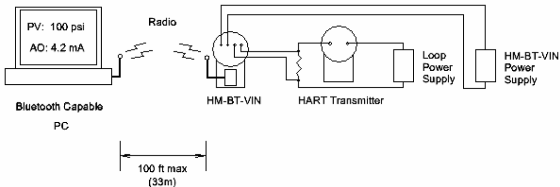
Figure 1. Typical Bluetooth System Diagram
